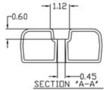
Common dimensions for 2, 3 and 4' models
